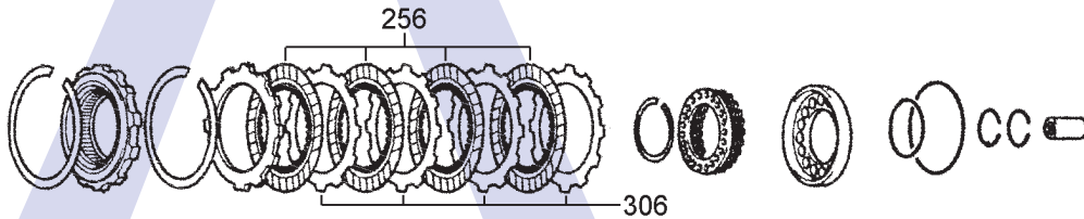
No.2 One-Way-Clutch (F2) & Underdrive Brake (B3) Assembly
